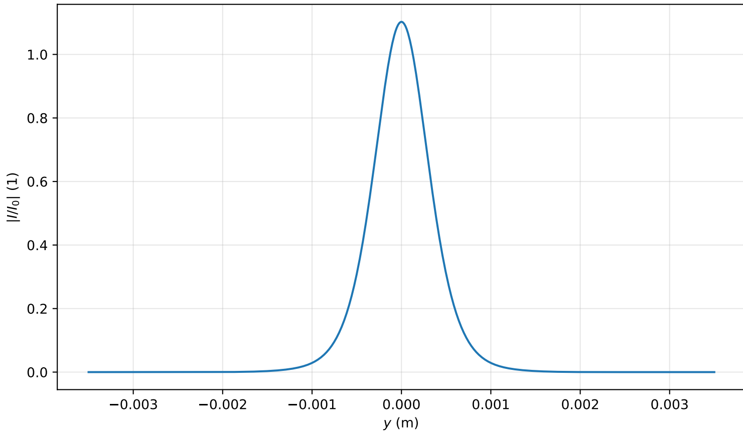
Intensity profile I(x=0, y, z=1.990)/I_0 , P_{in}=0.7P_{cr} , artificial time
